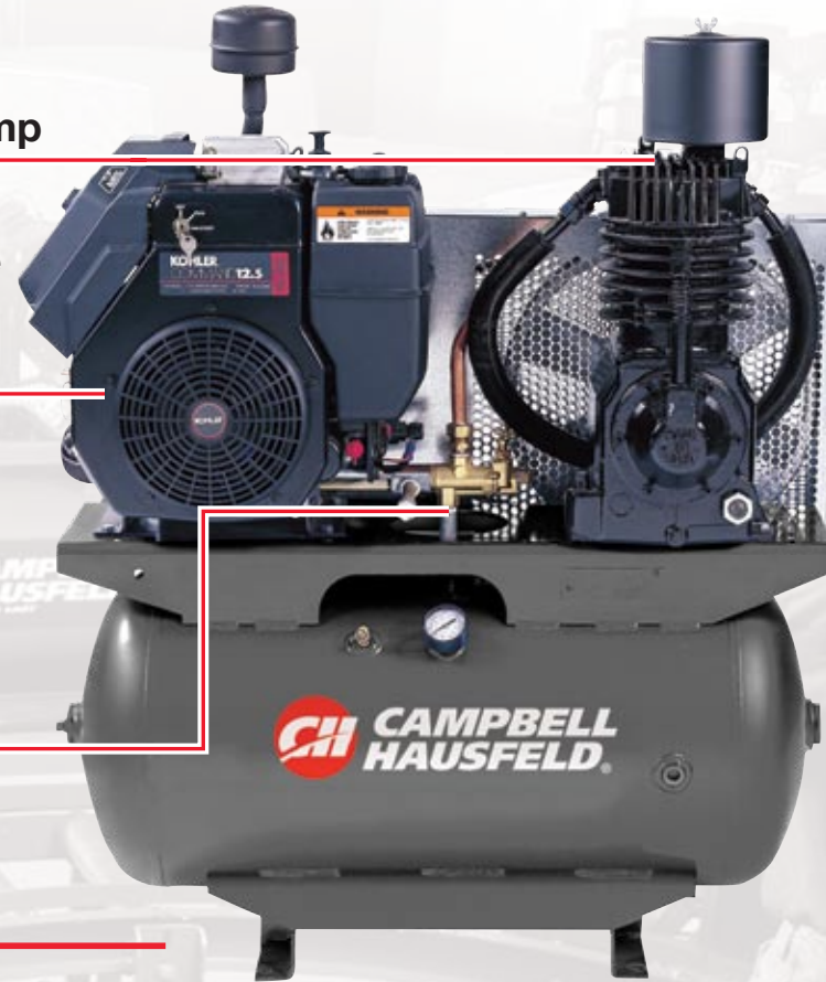
12.5HP Kohler Engine with Electric Start and Alternator
